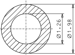
AL. TUBE
